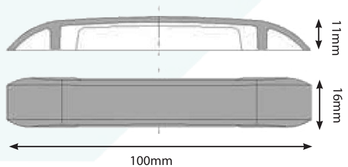
Drawing - Dimensions
