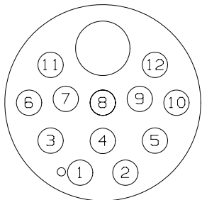
CONTACT VIEW
