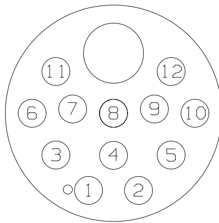
CONTACT VIEW
